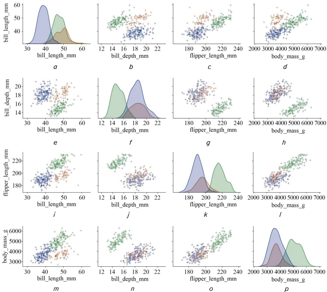
Fig. 1. Class distribution limit chart: ● – Chinstrap, ● – Adélie, ● – Gentoo
