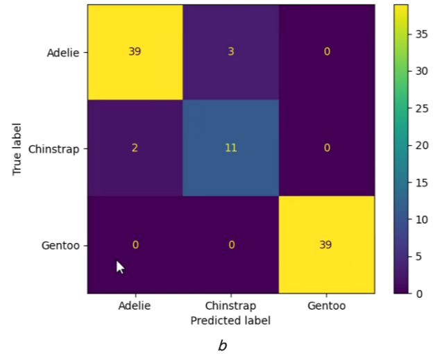
Fig. 6. Contradiction matrices – 250/94 (training/test): a – before training; b – after training
